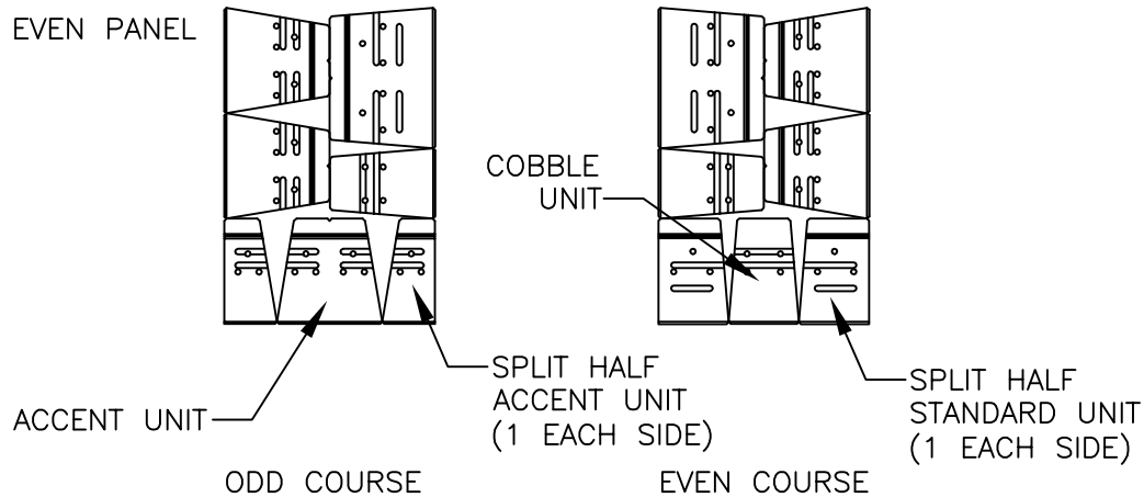
FREESTANDING BACK TO BACK MOSAIC UNITS - END WALL PLAN VIEW SCALE: NONE
