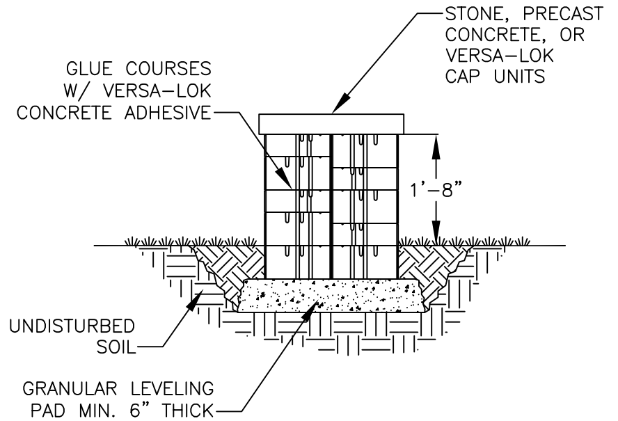
FREESTANDING BACK TO BACK MOSAIC UNITS - TYPICAL SECTION SCALE: NONE
