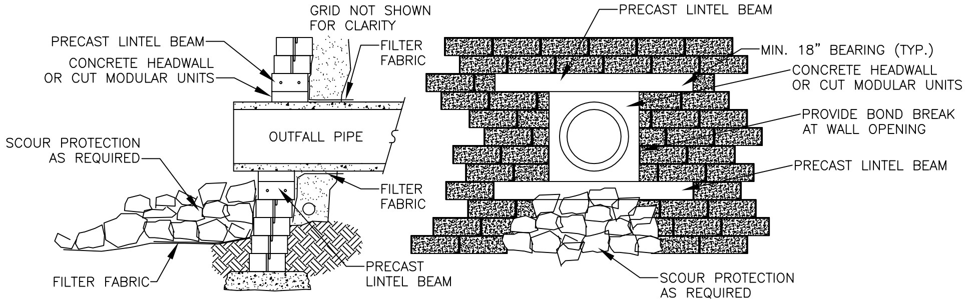
WALL W/ PIPE PENETRATION
