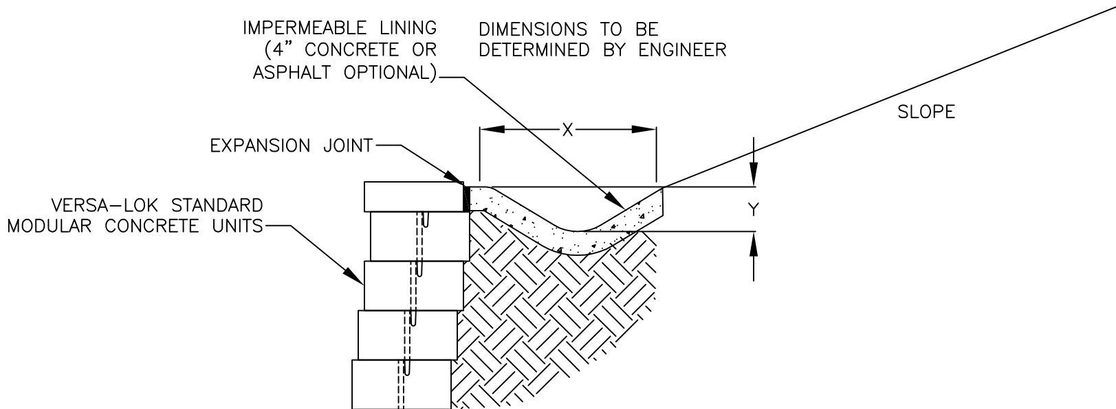
SWALE AT TOP OF WALL (OPTIONAL) SLOPE AT TOP OF WALL SCALE: NONE
