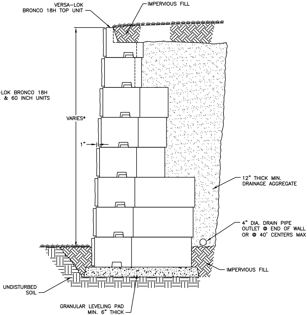
BRONCO 18H UNREINFORCED RETAINING WALL 24, 41, & 60 INCH UNITS SCALE: NONE
