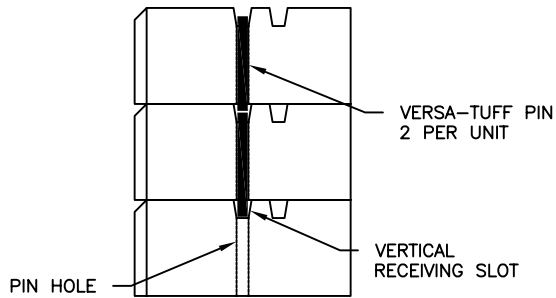
VERTICAL WALL PINNING DETAIL SCALE: NONE
