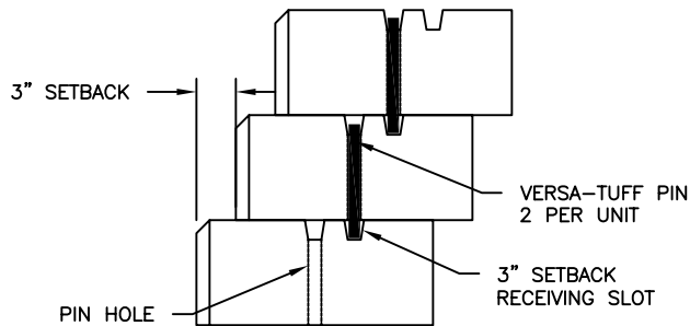
3" SETBACK PINNING DETAIL SCALE: NONE
