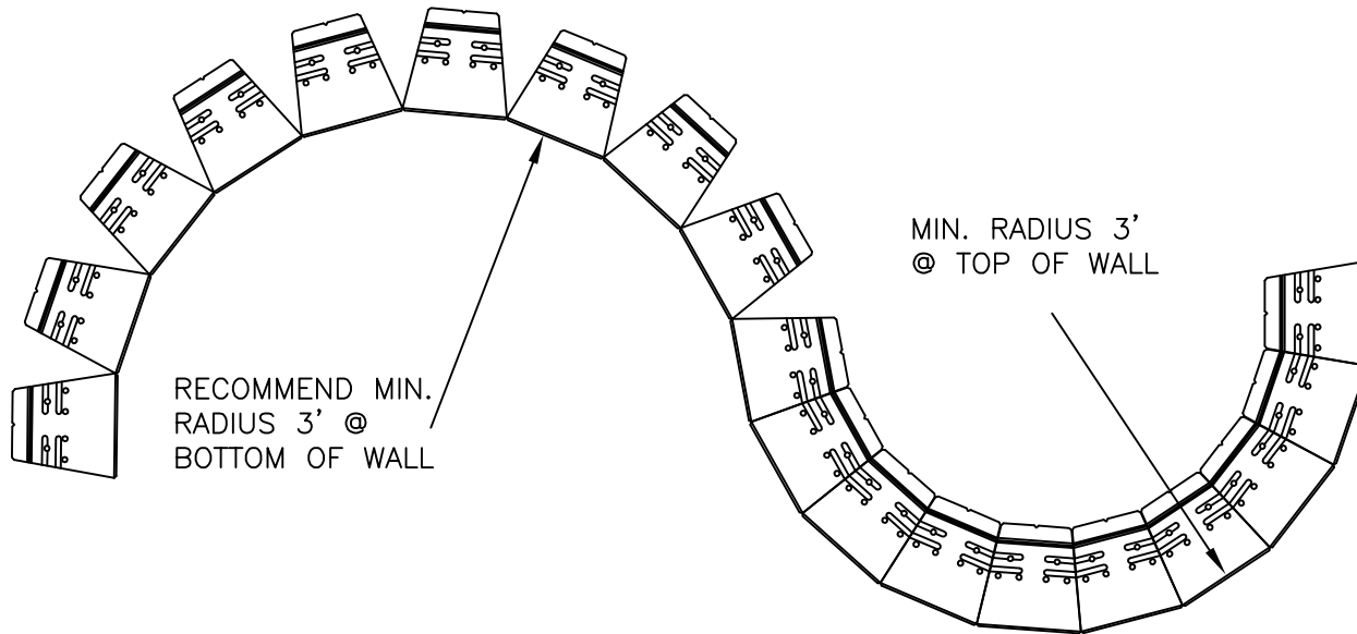
CURVE DETAIL ACCENT UNIT-TYPICAL CURVES SCALE: NONE
