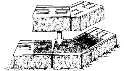
FIGURE 13A Large Angle Inside Corner (Optional)
