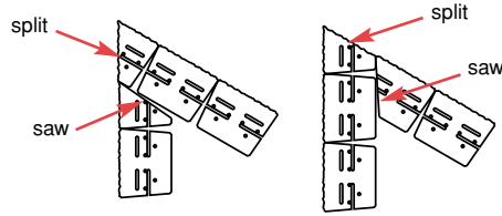
FIGURE 10 Low Angle Outside Corner
