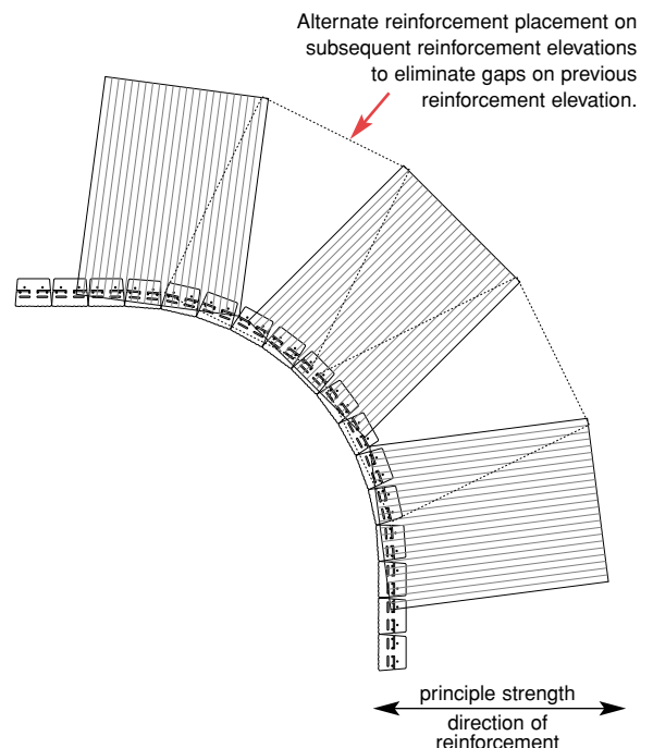
FIGURE 4 Concave Curve
