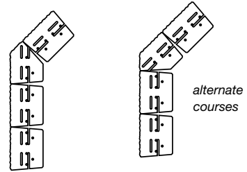
FIGURE 9 Large Angle Outside Corner
