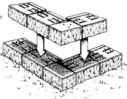
FIGURE 5 Outside 90° Corner
