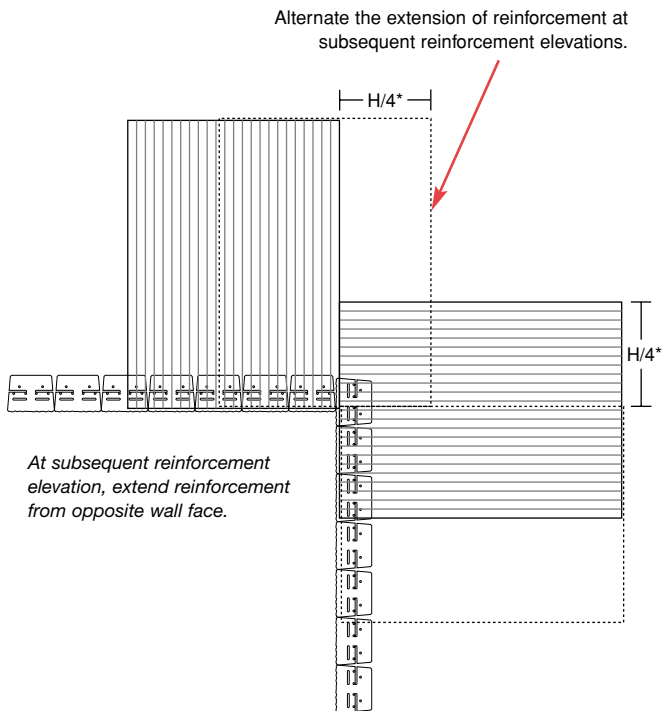
FIGURE 8 Inside Corner
