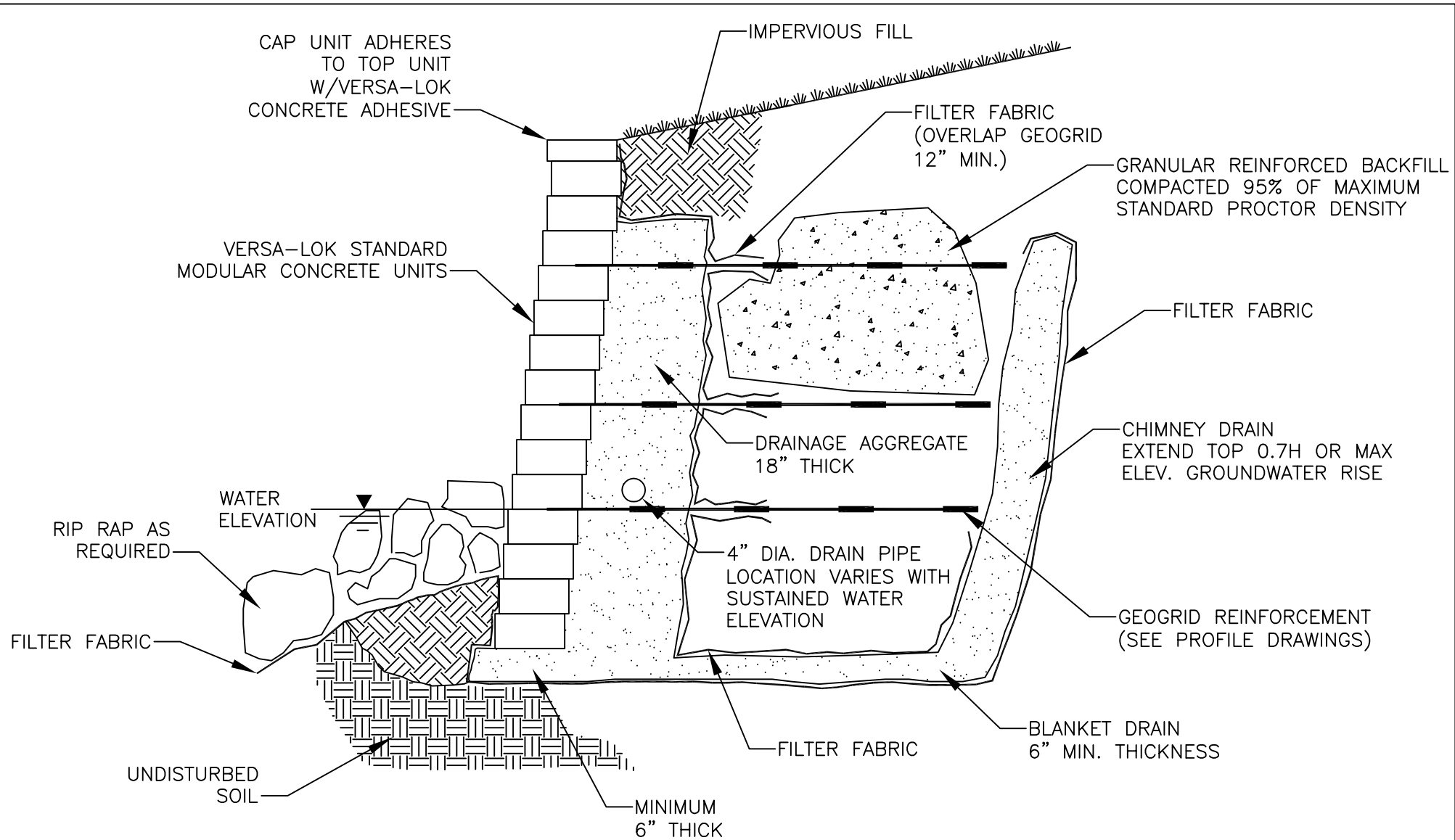
TYPICAL SECTION—REINFORCED SHORELINE WALL WITH BLANKET AND CHIMNEY DRAIN SCALE: NONE
