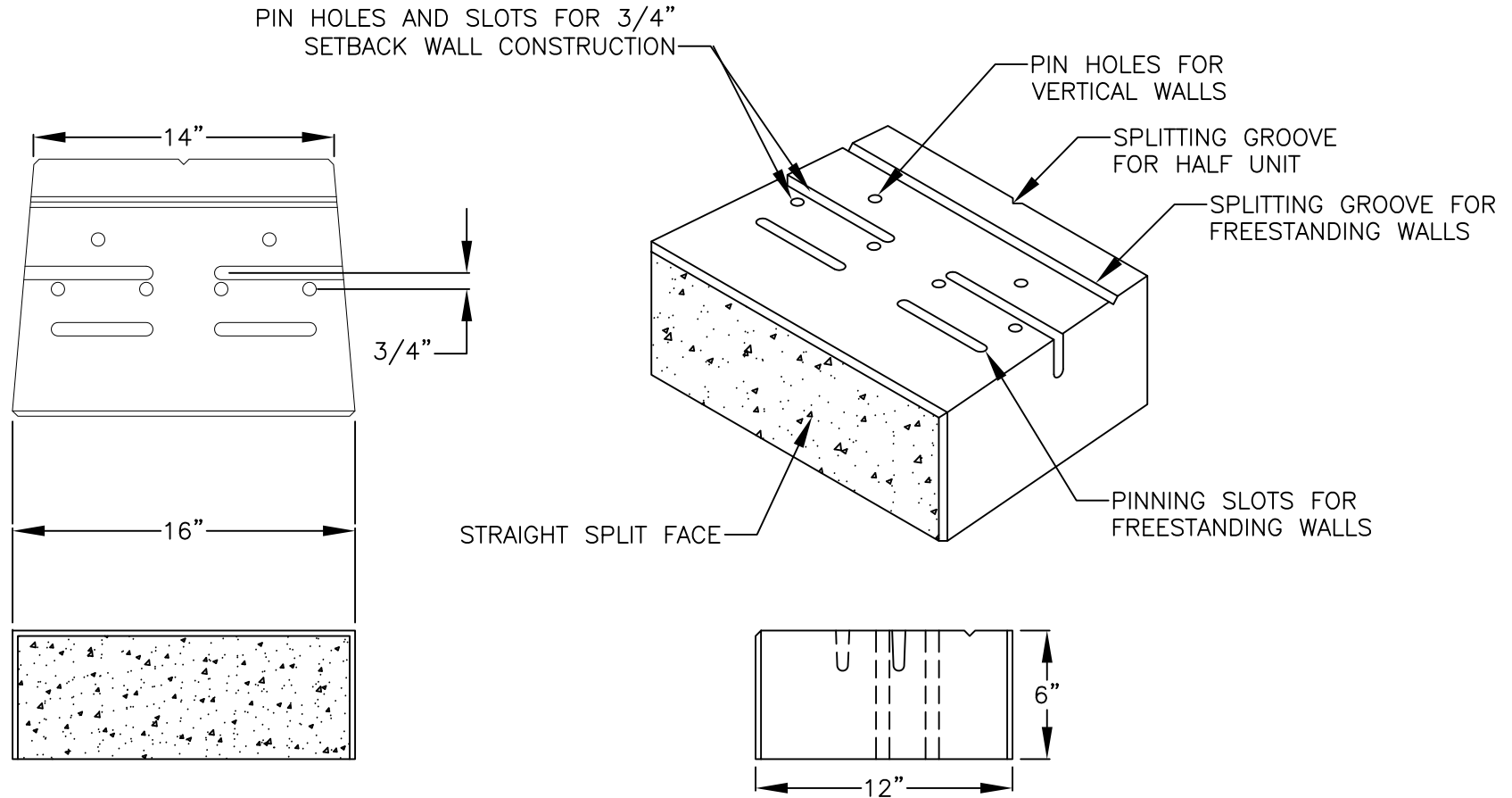
VERSA-LOK UNIT UNIT DIMENSIONS SCALE: 1-1/2"=1'
