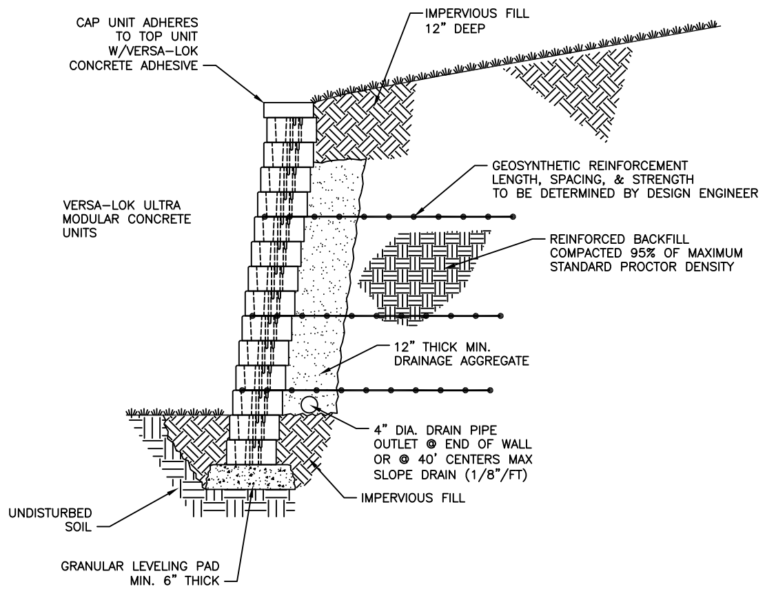
TYPICAL SECTION – REINFORCED RETAINING WALL SCALE: 3/8"=1'
