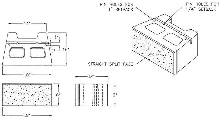
VERSA-LOK SQUARE FOOT UNIT
